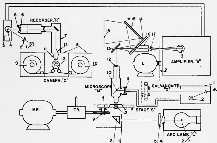
FIG. 1. Scheme of the graininess photometer: (The numbers refer to the various parts of each unit designated with a capital letter).
